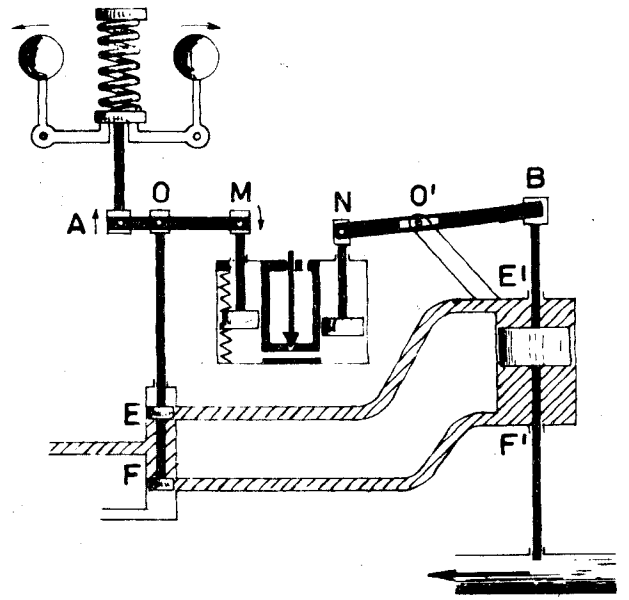
Fig. II / 24. Verhoging van belasting. (faze III).
