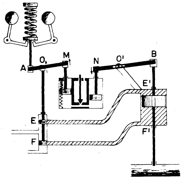
Fig. II / 23. Verhoging van belasting. (faze II).
